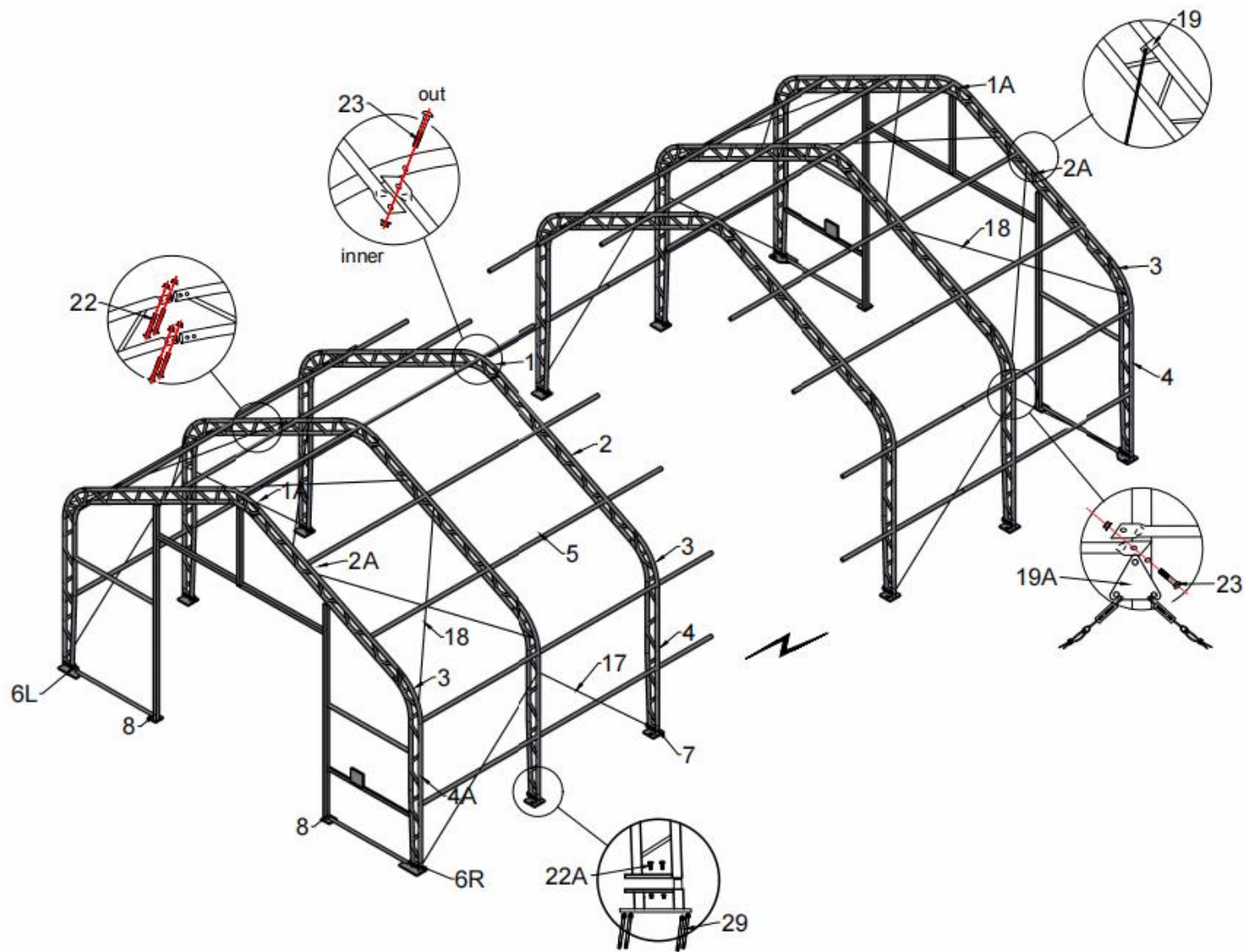
Figure 1: Frame Sketch
